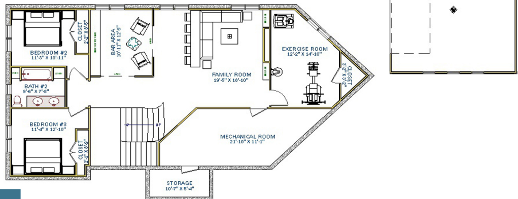
BASEMENT LEVEL FLOOR PLAN 1,504 FINISHED SQ. FT.
