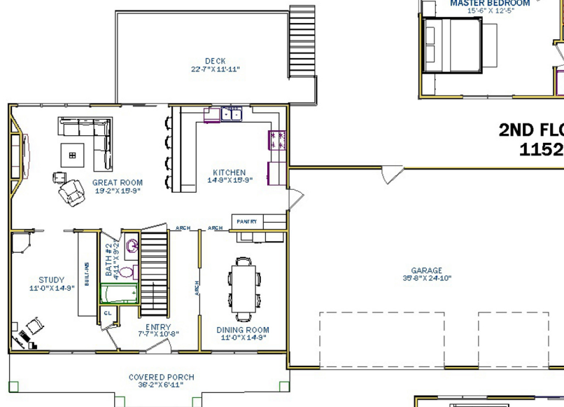
MAIN FLOOR PLAN 1152 SQ. FT.
