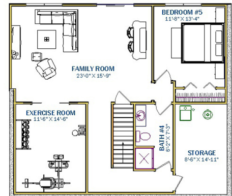
BASEMENT FLOOR PLAN 1019 FINISHED SQ. FT.
