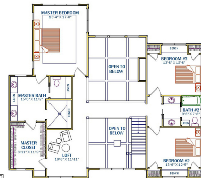
2ND FLOOR PLAN 1308 SQ. FT.
