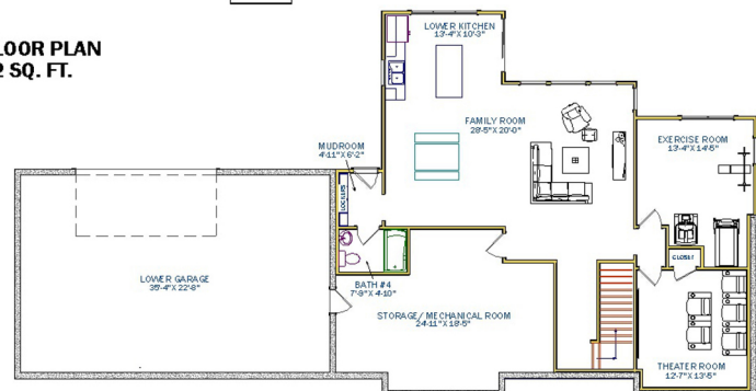
BASEMENT FLOOR PLAN 1320 SQ. FT. FINISHED
