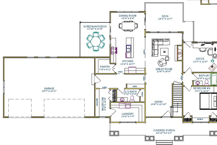
MAIN FLOOR PLAN 1712 SQ. FT.
